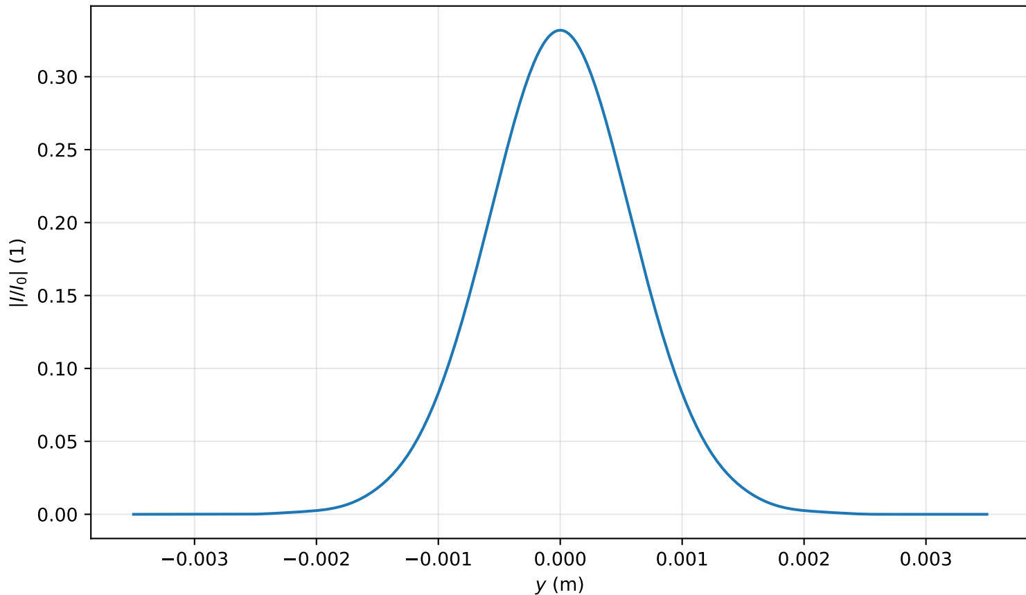
Intensity profile I(x=0, y, z=3.582)/I_0 , P_{in}=0.3P_{cr} , artificial time
